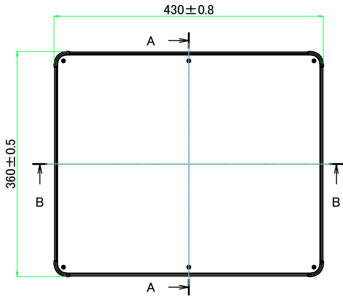
A view
